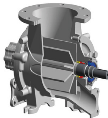
Cutaway of Coperion rotary airlock
